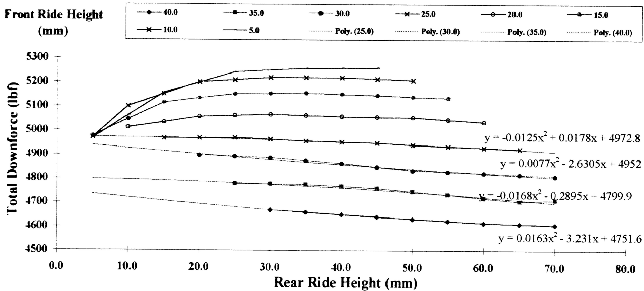
Total Downforce against Rear Ride Height at constant Front Ride Height
