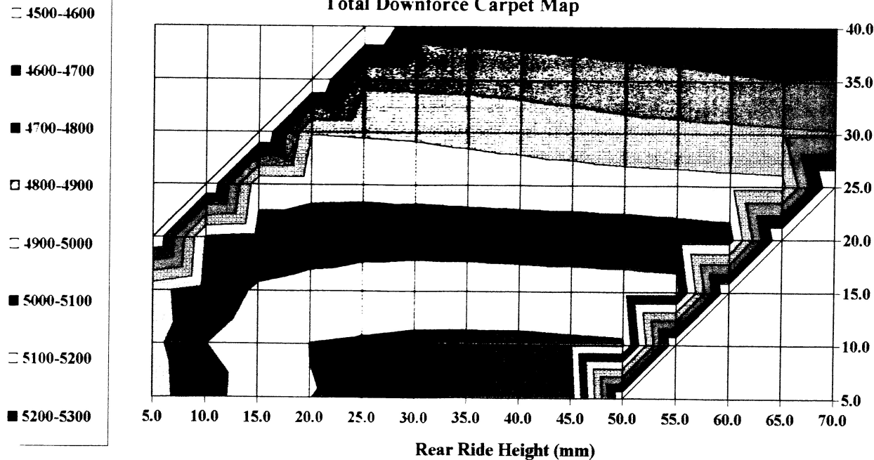
Total Downforce Carpet Map
